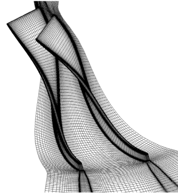
Fig. 2 Computational grid
