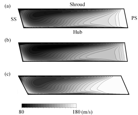
Fig. 8 Relative velocity distribution at the impeller exit (a) Case 1, (b) Case 3, and (c) Case 5
