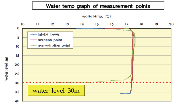
Fig. 9 Temp. changes of aeration, non-aeration and intake tower
