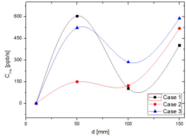
Fig. 6 Concentrations of Methyl Salicylate with U_i=1\text{ m/s}
