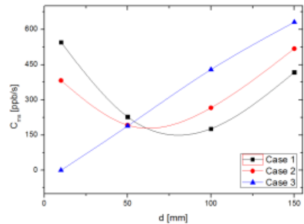
Fig. 7 Concentrations of Methyl Salicylate with U_i=2\text{ m/s}
