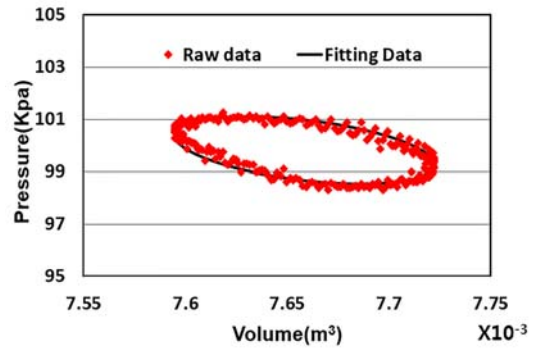
Fig. 6 Pressure-Volume diagram of the test Stirling engine (Condition: 75 ml/min, 82 °C, no load)
