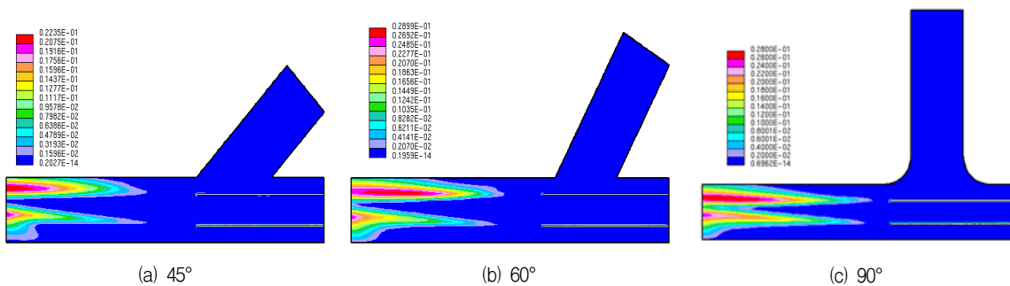
Fig. 6 Turbulent kinetic energy (V=1 m/s)
