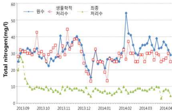
Fig. 5 Concentration(mg/L) of TN in the treated effluents by this wastewater treatment system
