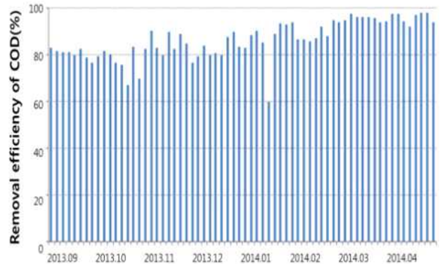
Fig. 3 Removal efficiency(%) of COD by this wastewater treatment system
