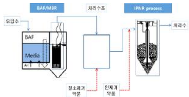
Fig. 1 Schematic diagram of wastewater treatment system
