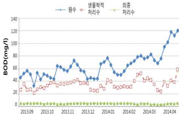
Fig. 2 Concentration(mg/L) of BOD in the treated effluents by this wastewater treatment system
