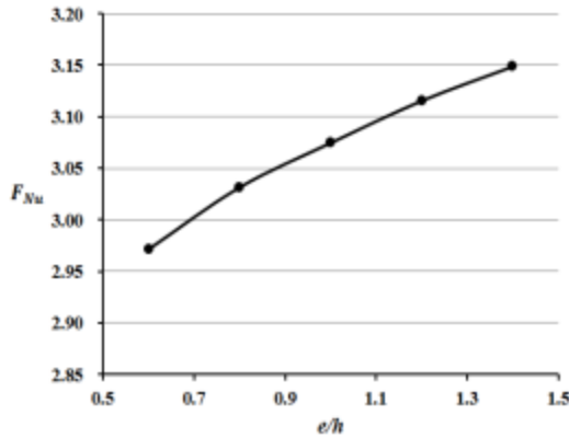
Fig. 16 Variation of F_{Nu} with rib width-to-height ratio
