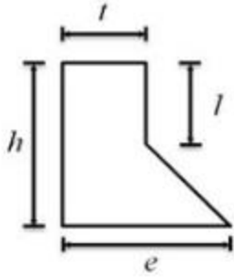
Fig. 3 Geometric parameters of a boot-shaped rib
