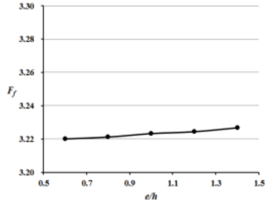
Fig. 17 Variation of F_f with rib width-to-height ratio
