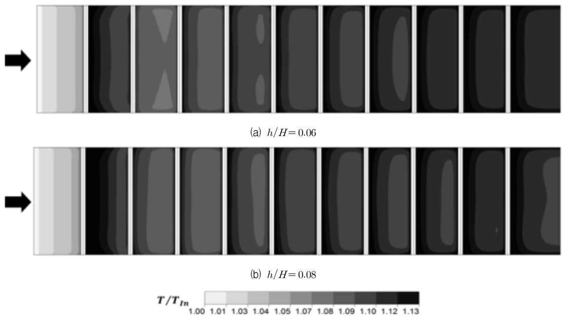
Fig. 14 Temperature distributions on the heated surface for different rib height-to-channel height ratios
