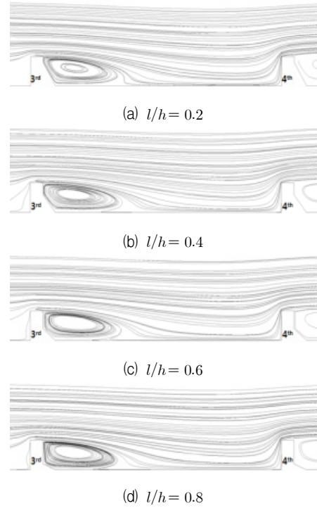
Fig. 10 Streamlines between third and fourth ribs on x-z plane for different l/h
