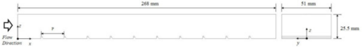
Fig. 1 Geometry of ribbed cooling channel.
