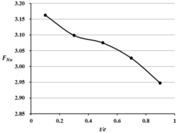
Fig. 4 Variation of F_{Nu} with tip width-to-rib width ratio
