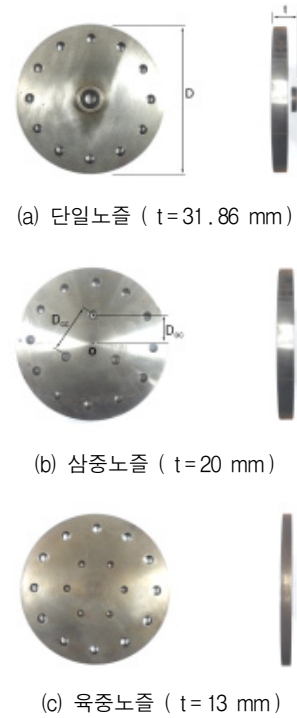
Fig. 1 Experimental model with supersonic nozzle
