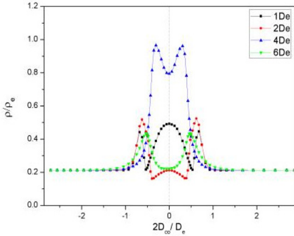
Fig. 9 Comparison of density for three nozzles
