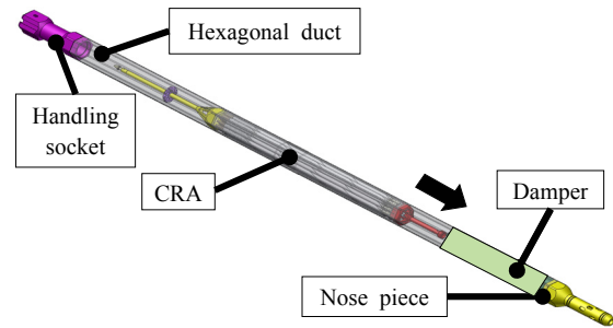
Fig. 1 Configuration of a guide duct and control rod assembly
