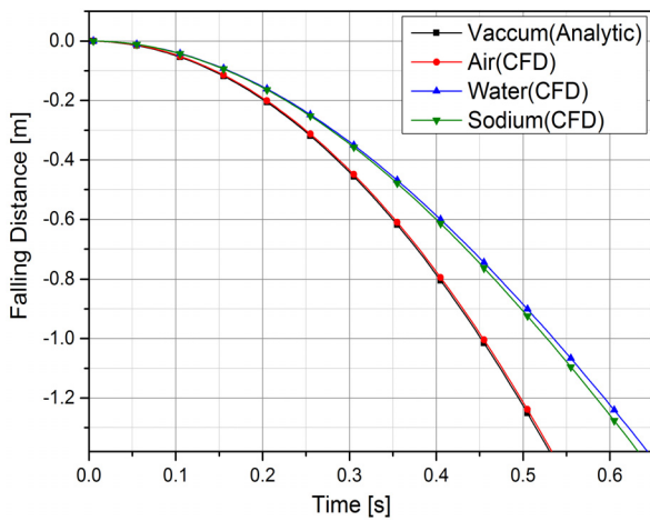
Fig. 5 Falling distance of a steel ball in various fluid
