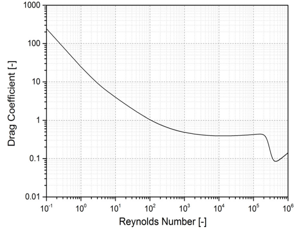
Fig. 6 Drag coefficient as a function of Reynolds number
