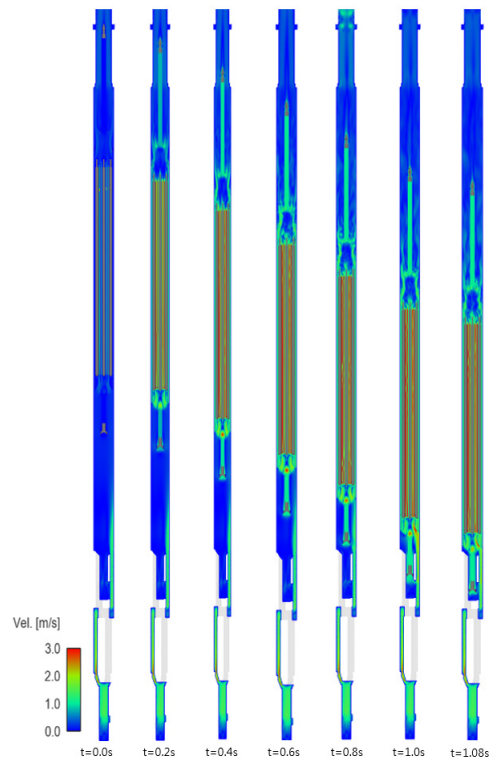
Fig. 9 Falling distance of a SFR control rod assembly
