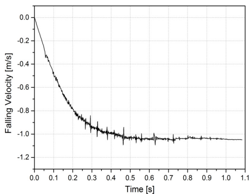
Fig. 11 Falling velocity of a SFR control rod assembly
