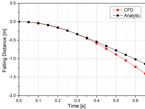
Fig. 7 Falling distance of a steel ball in water
