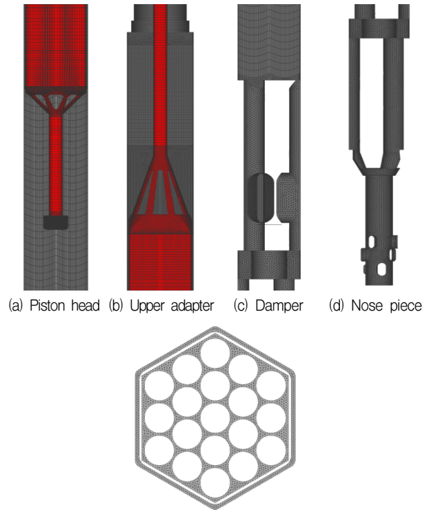
(e) Horizontal cross section of a control rod and hexagonal duct
