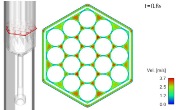
Fig. 12 Falling velocity of a SFR control rod assembly
