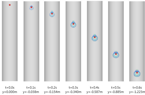
Fig. 4 Falling distance of a steel ball in various fluid
