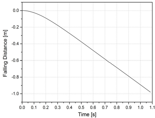
Fig. 10 Falling distance of a SFR control rod assembly
