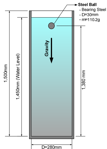
Fig. 3 Schematic drawing for free falling of a steel ball in water for methodology verification
