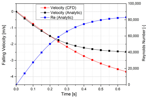
Fig. 8 Falling velocity and Reynolds number of a steel ball in water
